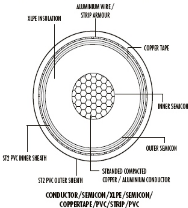
TYPICAL CONSTRUCTION OF POLY CAB 1 CORE HT XLPE CABLE
