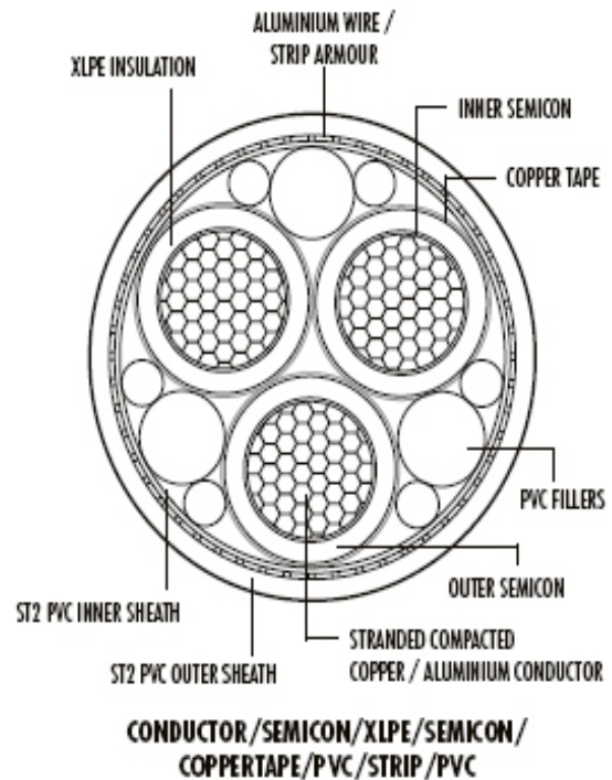
TYPICAL CONSTRUCTION OF POLY CAB 3 CORE HT XLPE CABLE
